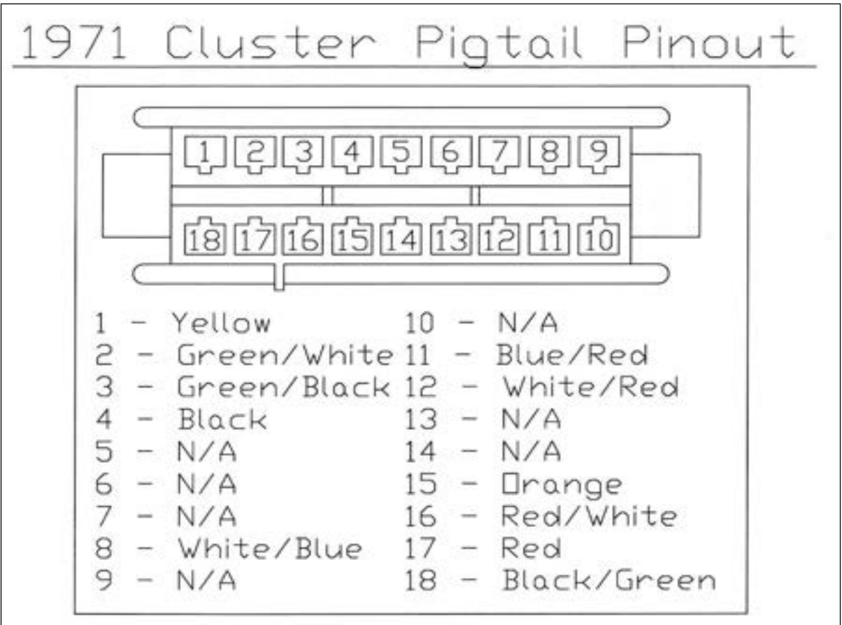
Figure 7-36 1971 (AND SOME 1972 MODELS) Cluster Pigtail Pinout
